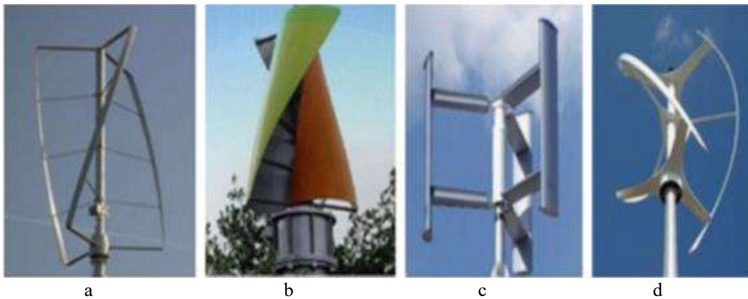
Gambar 6. VAWTs tipe darrieus (a) Turbin Turby, (b) Turbin WinSide, (c) Turbin Ropatec, dan (d) Turbin Gorlov Helical [10]
