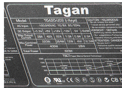
Gambar 4.16. Nameplate
