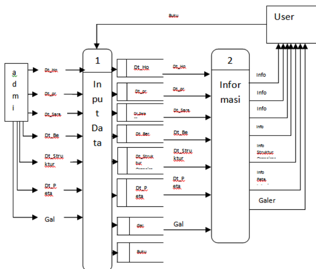
Gambar 2 DFD Level 0
