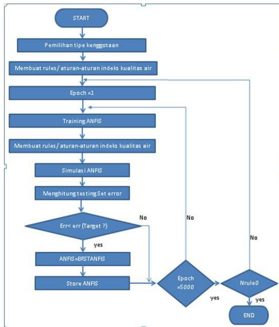
Gambar 2. Alur training ANFIS
