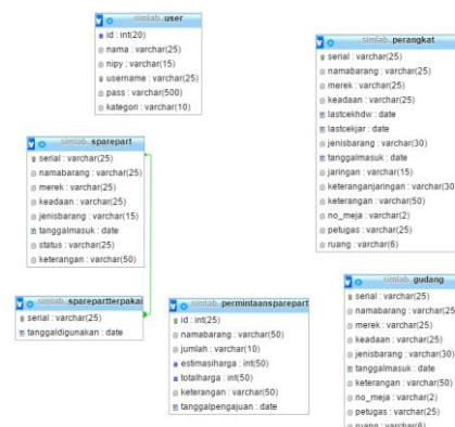
Gambar 4. Class Diagram
