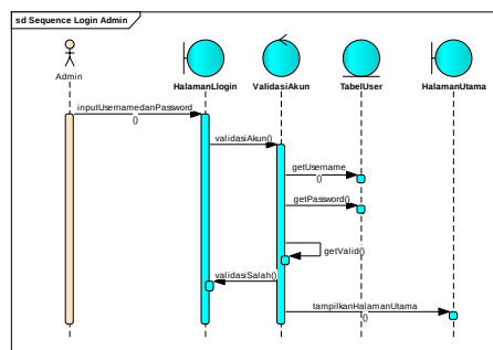
Gambar 3. Sequence Diagram Login
